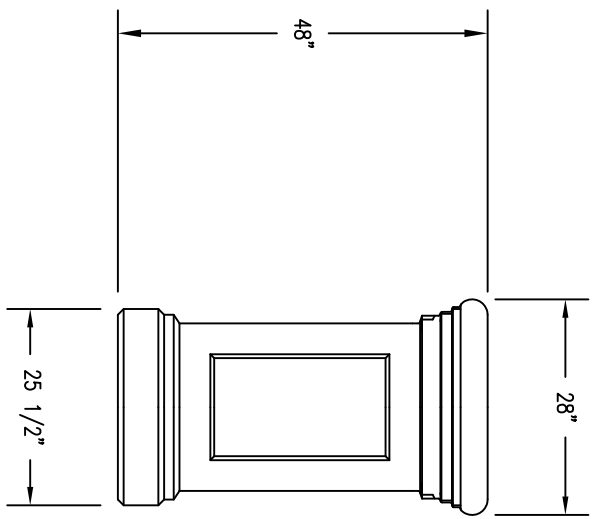
2 ELEVATION VIEW
