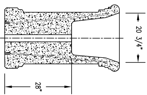
4 CROSS SECTION
