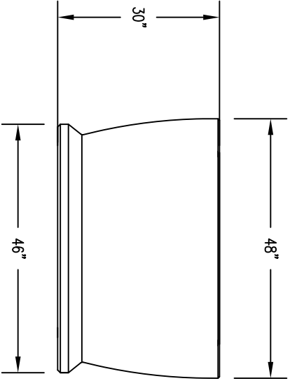
2 ELEVATION VIEW
