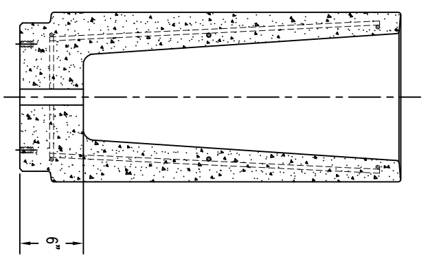
4 CROSS SECTION
